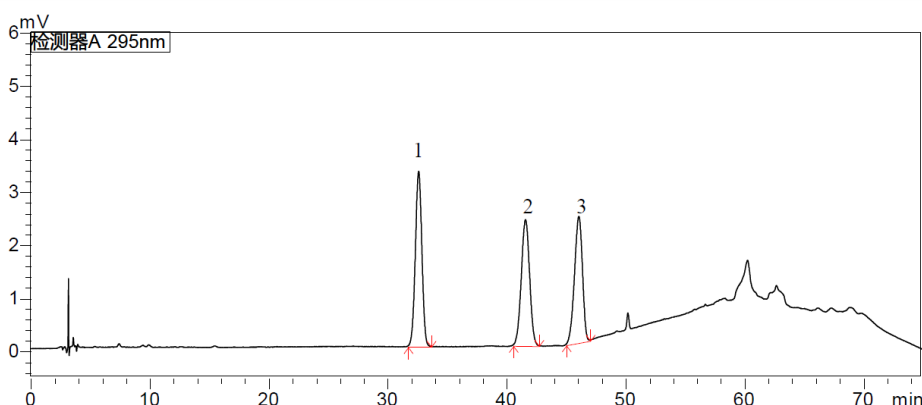
Chromatogram of System Suitability Solution
