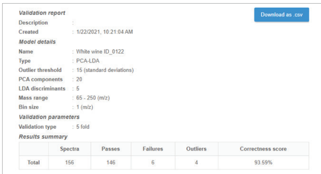
Figure 4. Cross validation results of the classification model of Baijiu flavor type based on RADIAN ASAP data.
