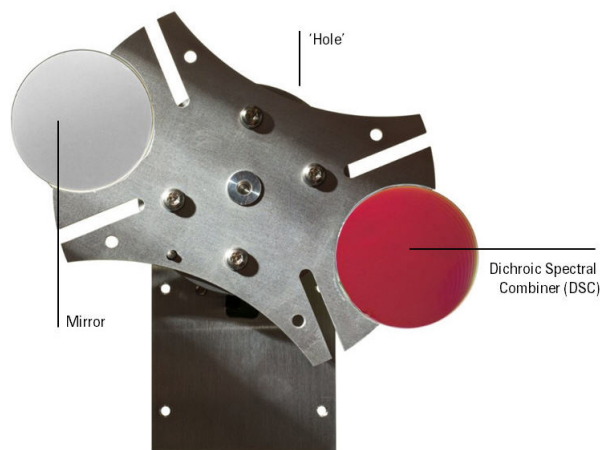
Figure 3. The mode selector component that enables the four modes of operation in the 5110 SVDV configuration.
