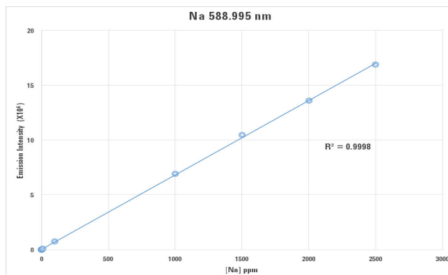
Figure 2. Na 589.995 nm, 0.1 - 2500 ppm Linear Dynamic Range when measured in SVDV mode.
